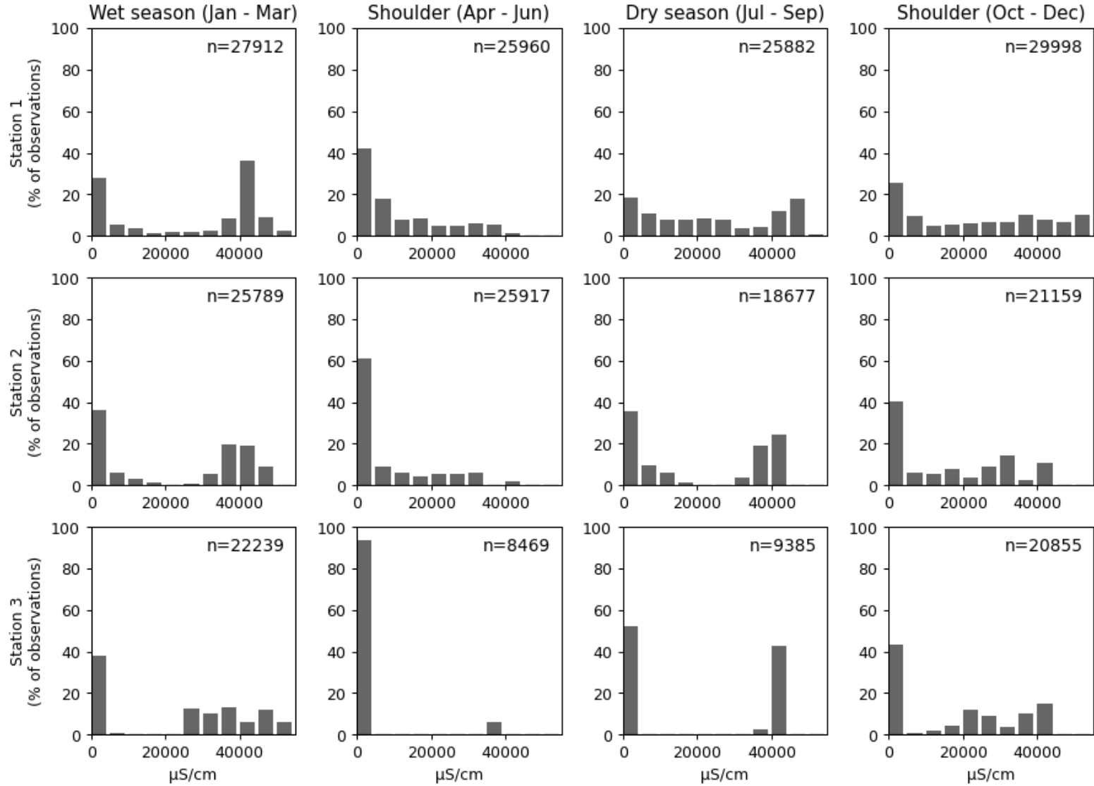
Figure B-2 Seasonal conductivity observations
