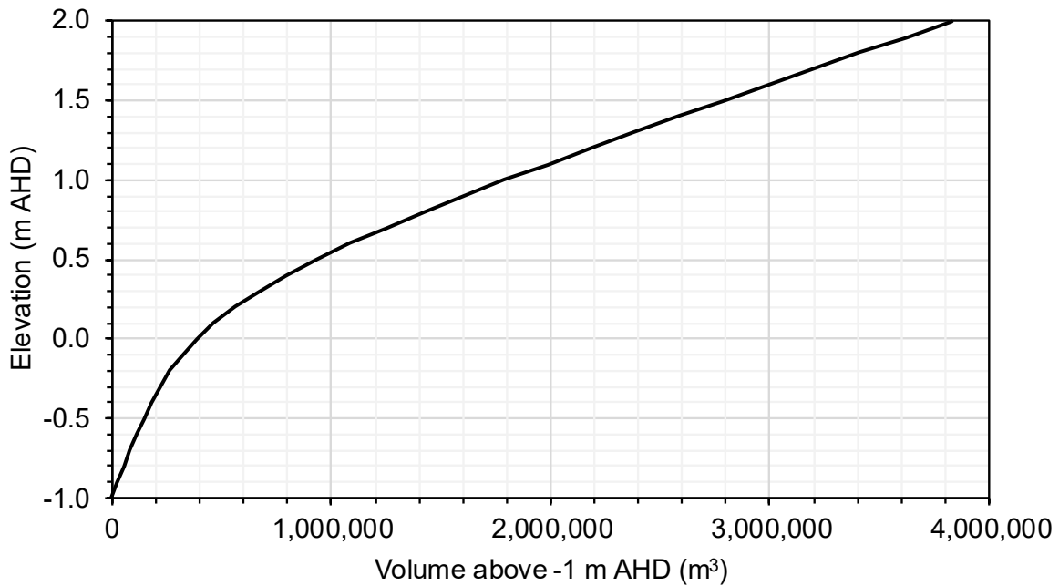
Figure 7-1 Volume of water in the Clybucca drainage network above -1 m AHD
