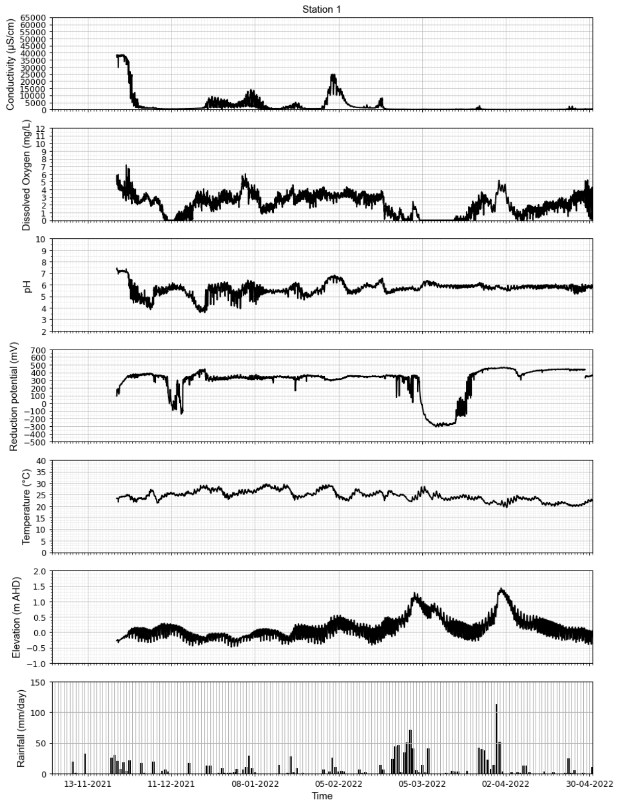
Figure A-1 Water quality data for Station 1 (November 2021 to April 2022)
