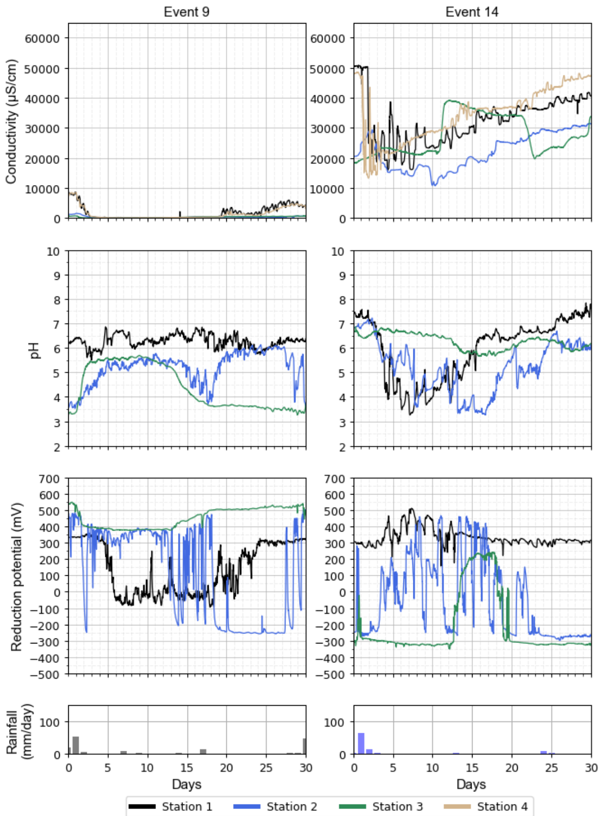
Figure C-5 Comparison of event 9 (22/9/2022) and event 14 (4/11/2023)
