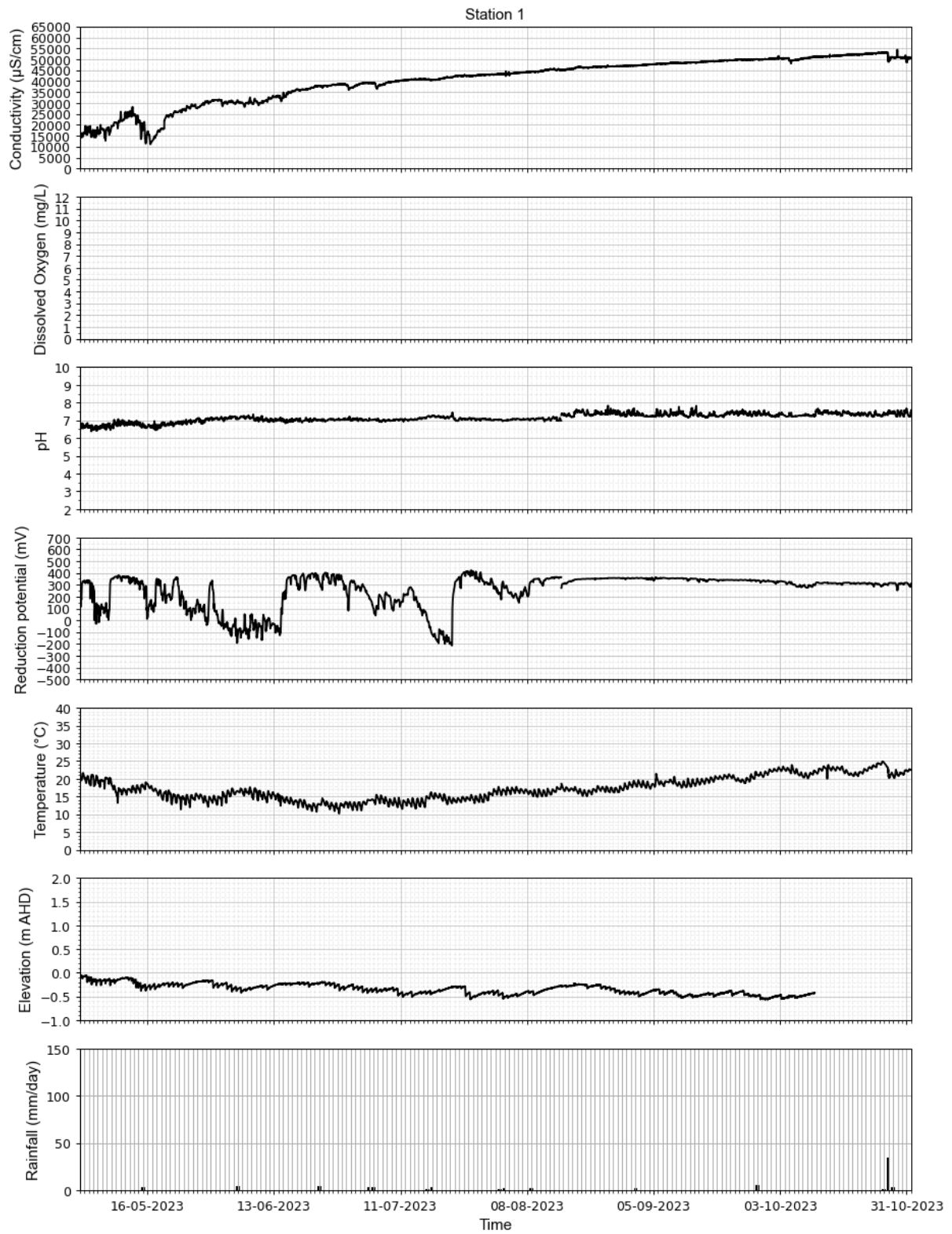
Figure A-4 Water quality data for Station 1 (May 2023 to October 2023)
