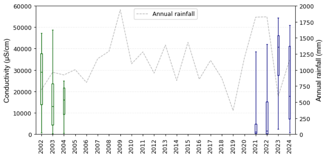
Figure 5-3 Conductivity measurements upstream of the Menarcobrinni floodgates as recorded by Greenspan (green) and the existing WRL monitoring program (blue)
