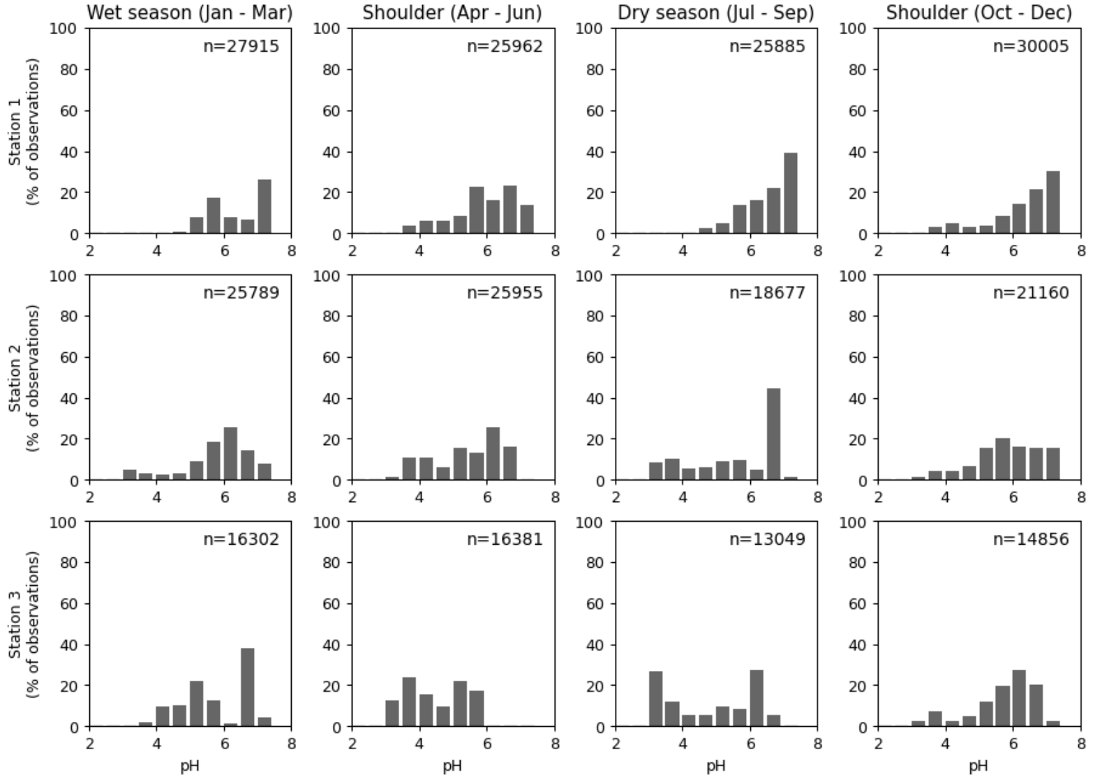
Figure B-3 Seasonal pH observations
