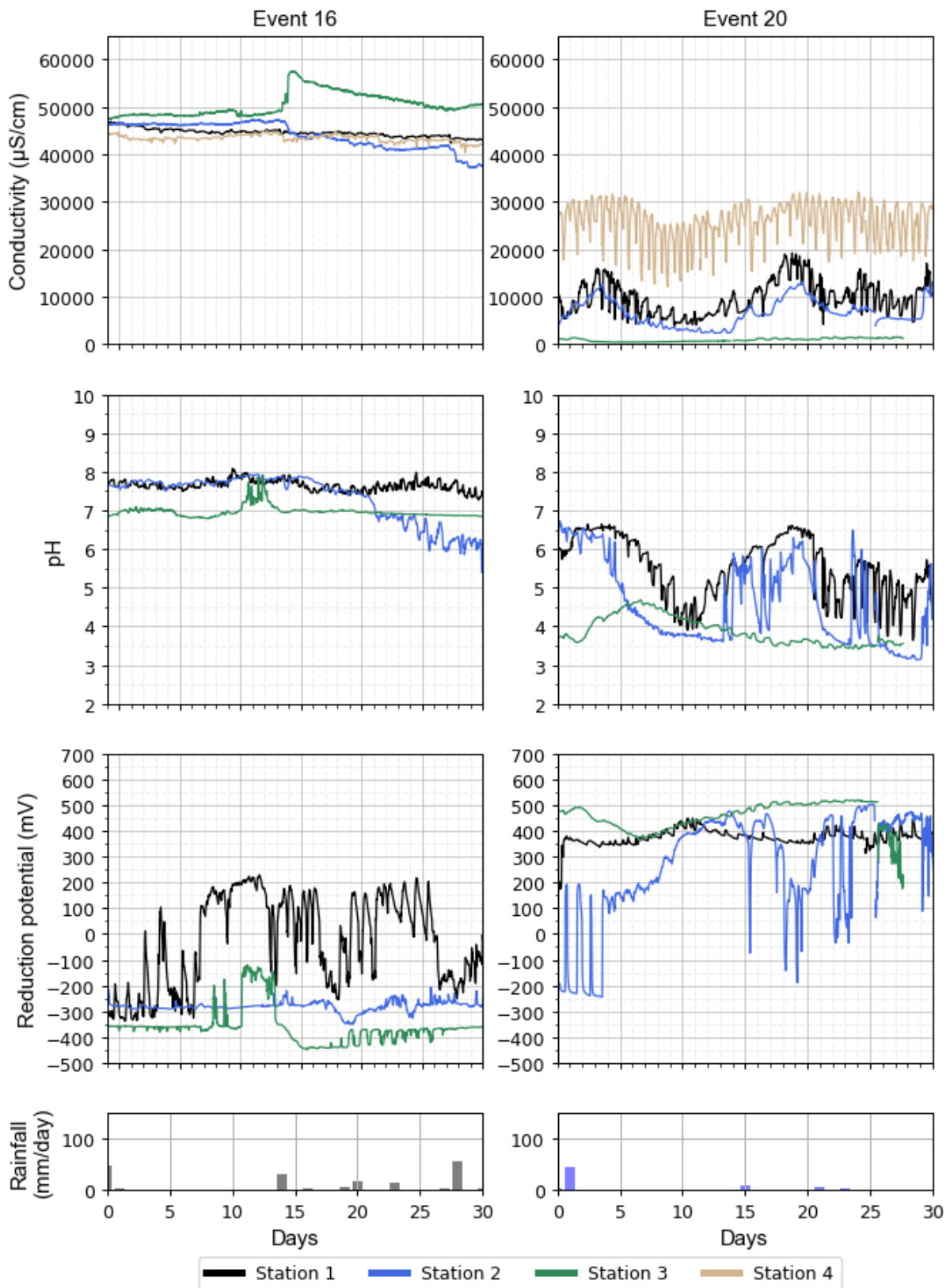
Figure C-6 Comparison of event 16 (28/1/2024) and event 20 (1/6/2024)
