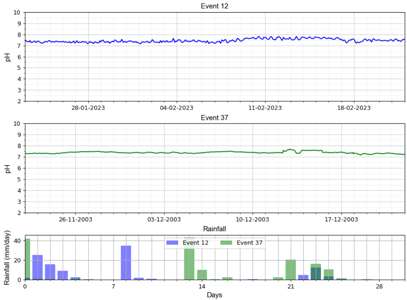
Figure C-9 Comparison of event 12 (23/01/2023) and event 37 (22/11/2003). Rainfall data from BOM (2025b)
