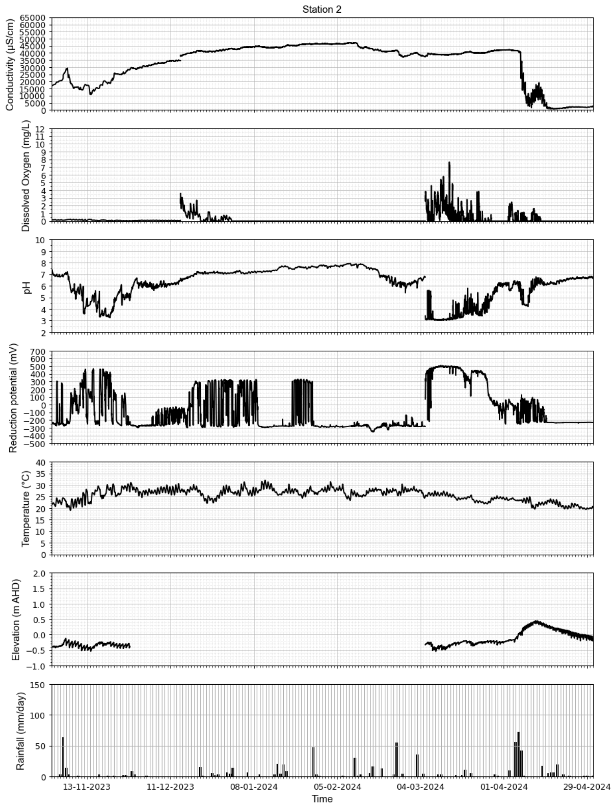
Figure A-12 Water quality data for Station 2 (November 2023 to April 2024)
