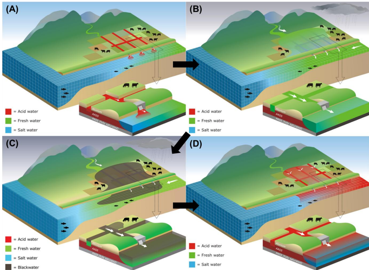
Figure 2-1 Hydrological influence on the water quality processes of coastal floodplains (adapted from Johnston et al. (2003) Ruprecht et al. (2018) and Waddington et al. (2022))
