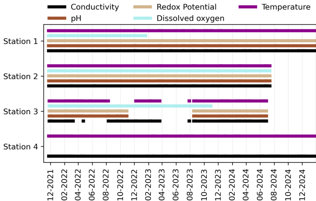
Figure 3-1 Times when water quality data was available for each station
