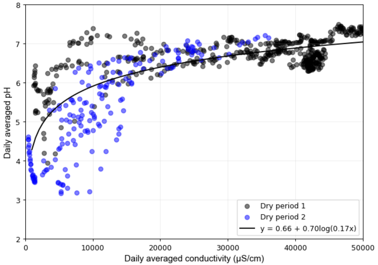
Figure 3-8 Daily averaged pH versus daily averaged conductivity for each dry period
