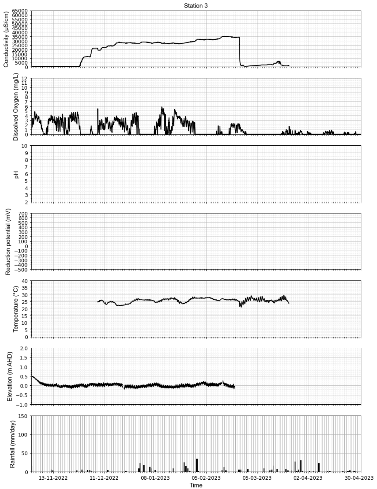
Figure A-16 Water quality data for Station 3 (November 2022 to April 2023)
