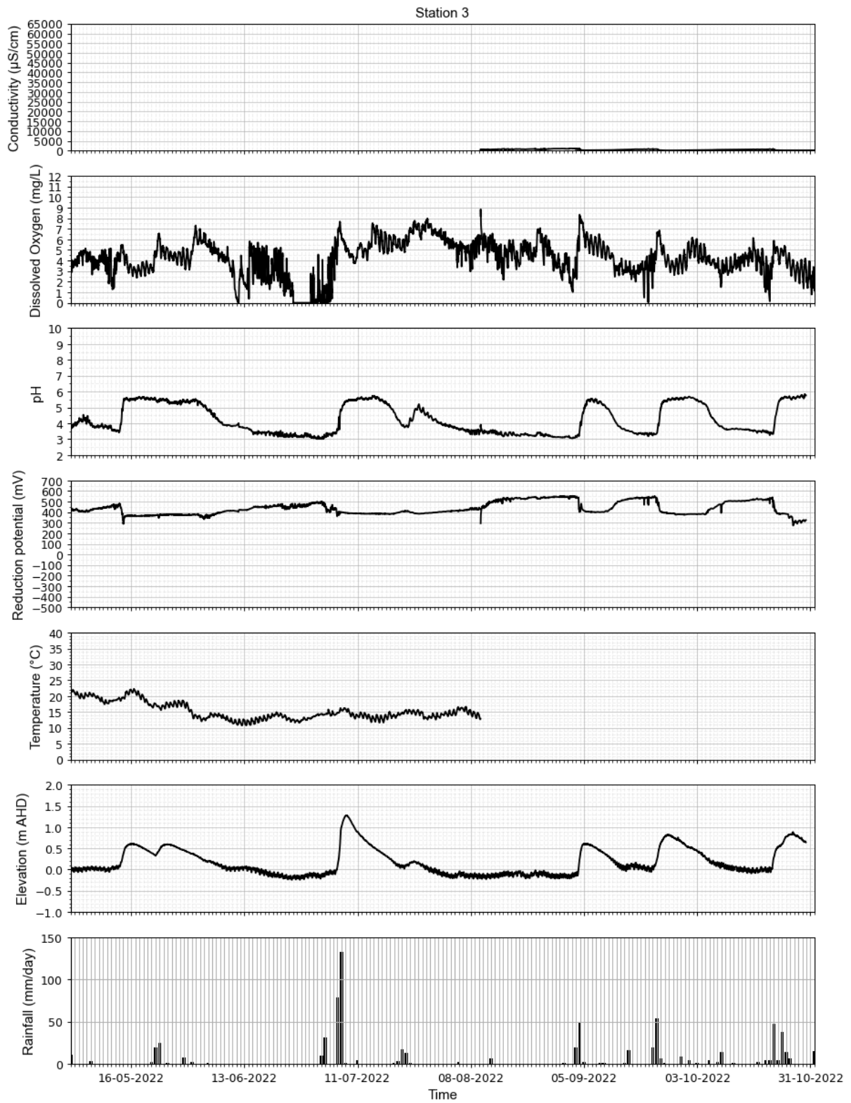
Figure A-15 Water quality data for Station 3 (May 2022 to October 2022)
