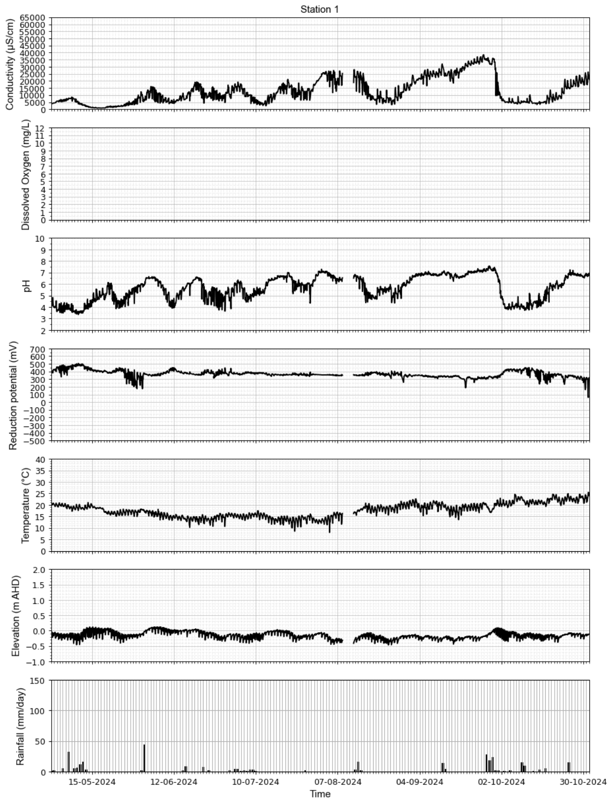
Figure A-6 Water quality data for Station 1 (May 2024 to October 2024) Rainfall data from BOM (2025e)
