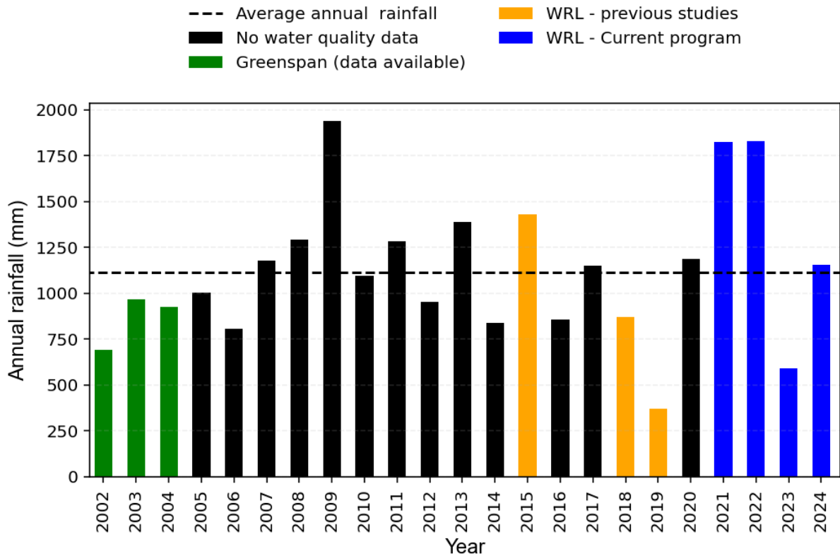
Figure 5-1 Comparison of annual rainfall for different years of water quality monitoring
