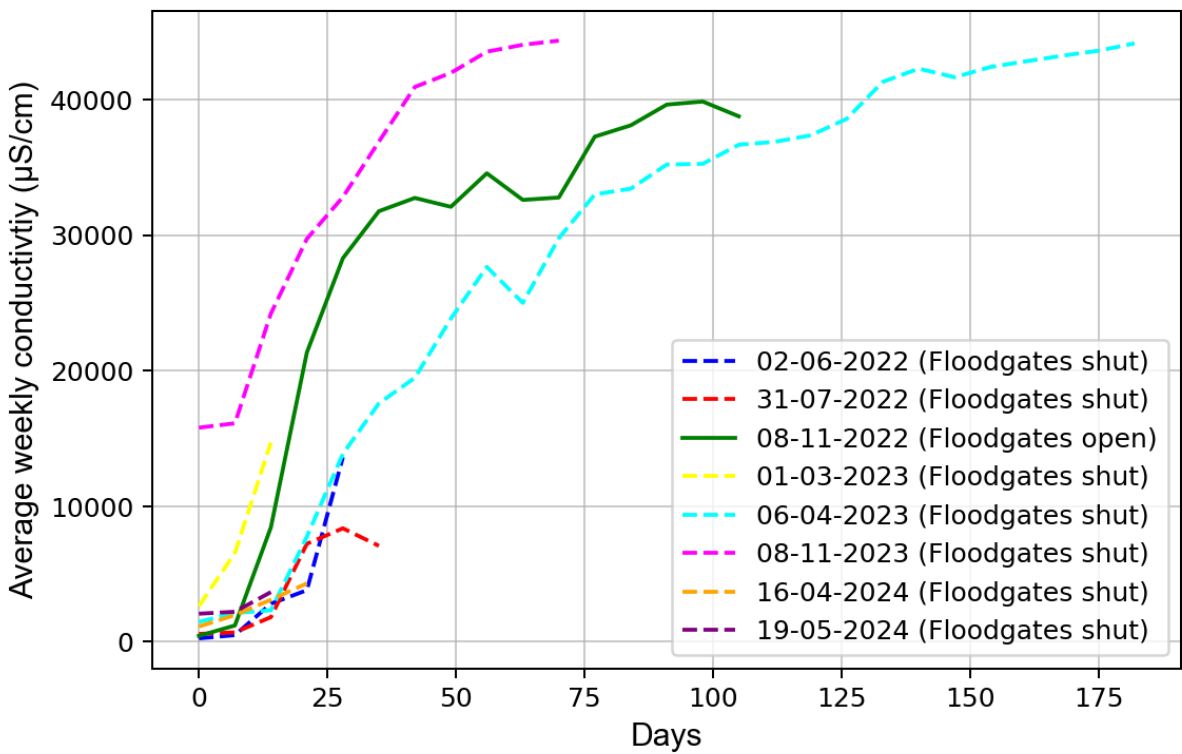
Figure 4-4 Comparison of conductivity increase due to tidal flushing Station 2 when two floodgates were opened versus shut
