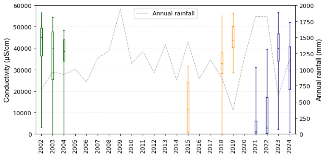
Figure 5-2 Conductivity measurements downstream of the Menarcobrinni floodgates as recorded by Greenspan (green), Glamore and Rayner (2017) and Rayner et al. (2020) (orange), and the existing monitoring program (blue)
