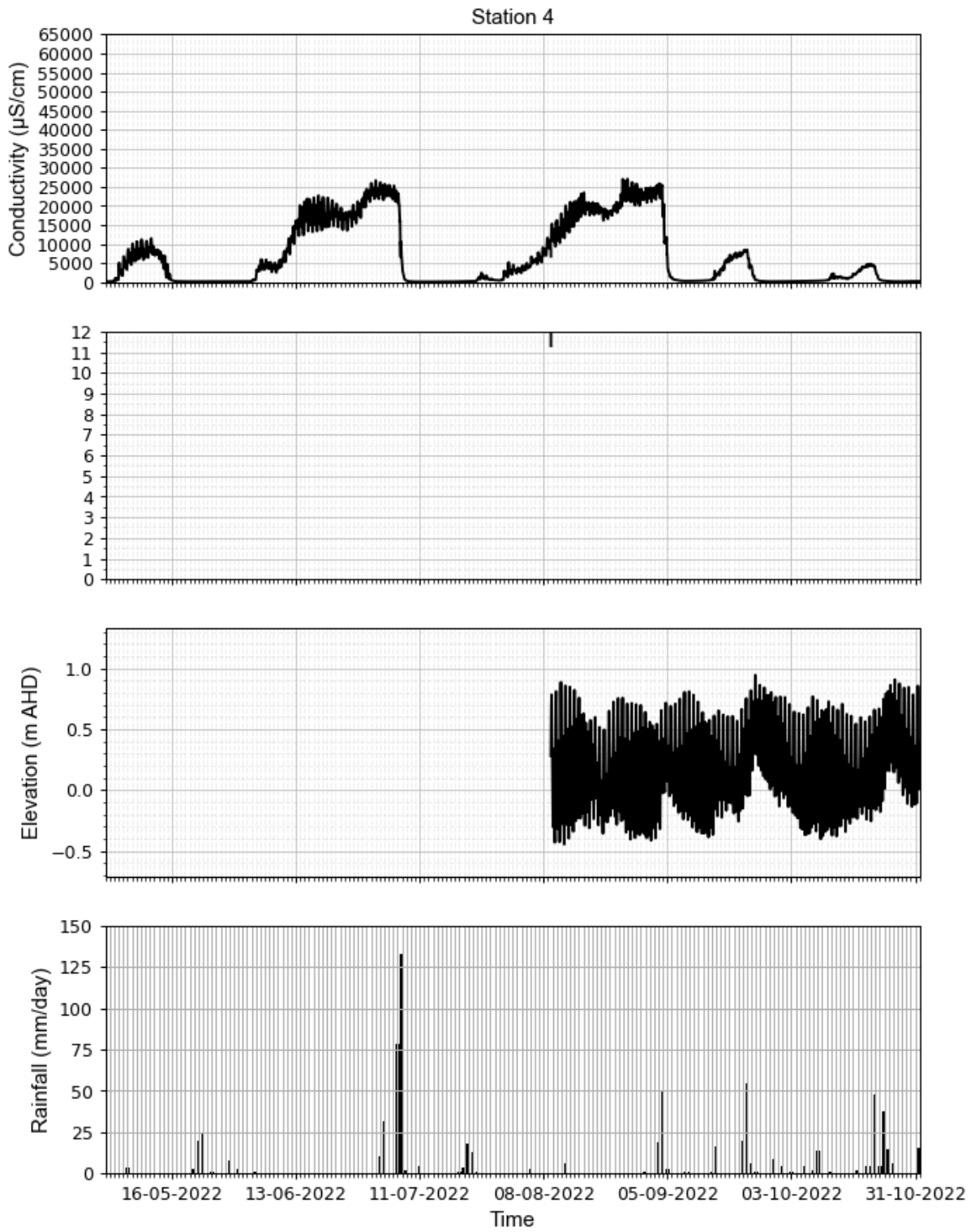
Figure A-21 Water quality data for Station 4 (May 2022 to October 2022)
