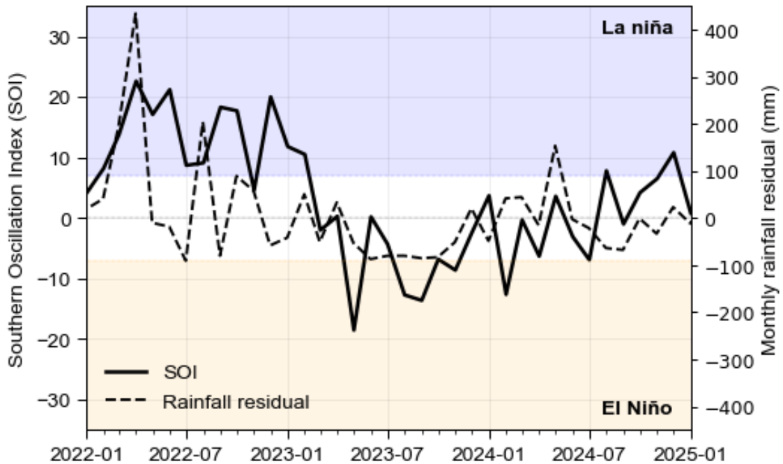
Figure 2-3 Residual rainfall (i.e. monthly rainfall minus the average monthly rainfall) compared to the Southern Oscillation Index (data accessed from BOM (2025e) and BOM (2025f))
