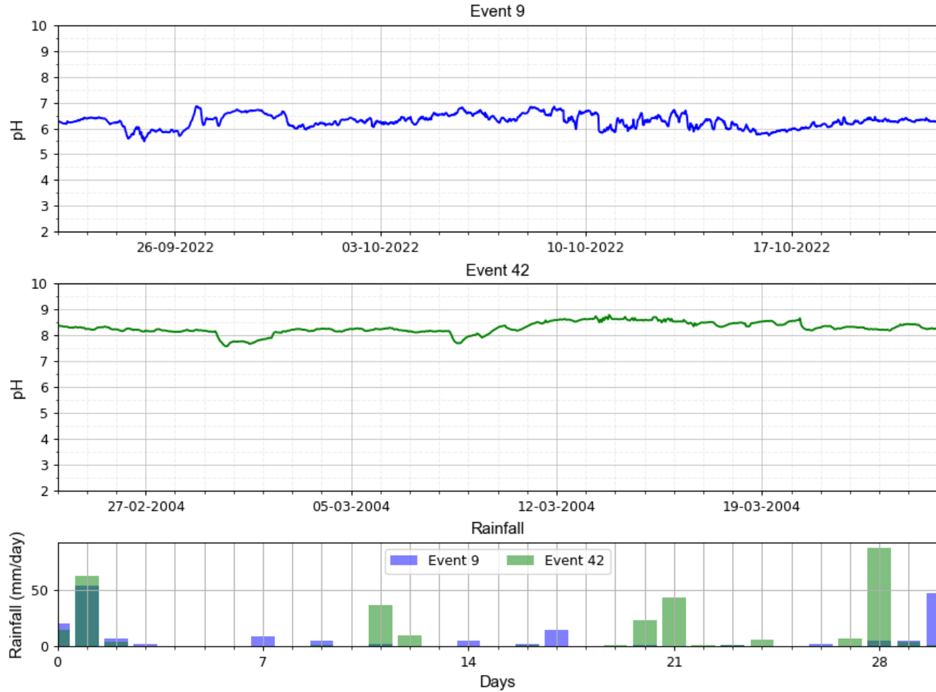
Figure C-8 Comparison of event 9 (22/09/2022) and event 42 (24/02/2004). Rainfall data from BOM (2025b)
