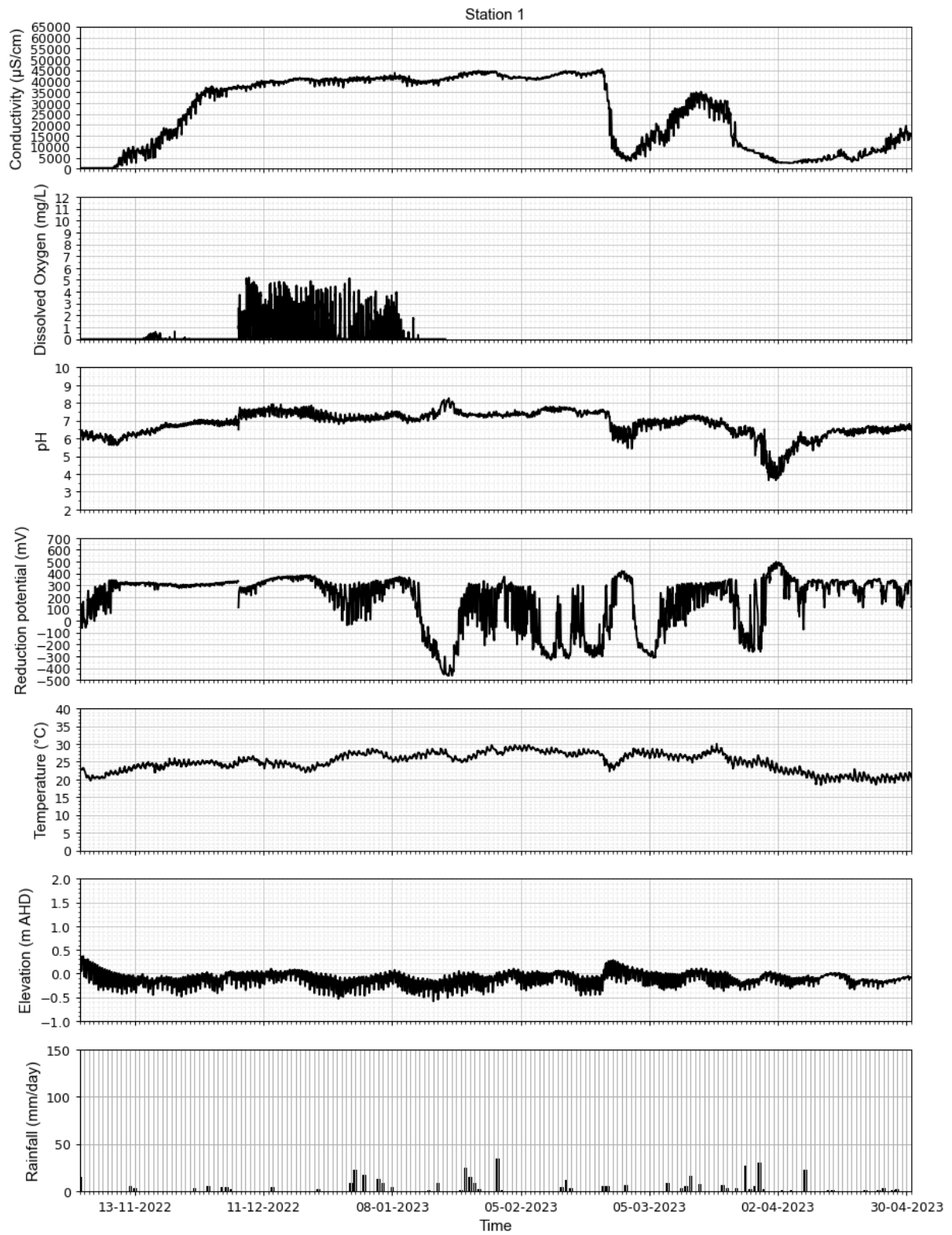
Figure A-3 Water quality data for Station 1 (November 2022 to April 2023)
