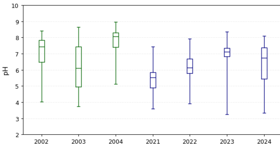
Figure 5-4 pH measurements upstream of the Menarcobrinni floodgates as recorded by Greenspan (green) and the existing monitoring program (blue)
