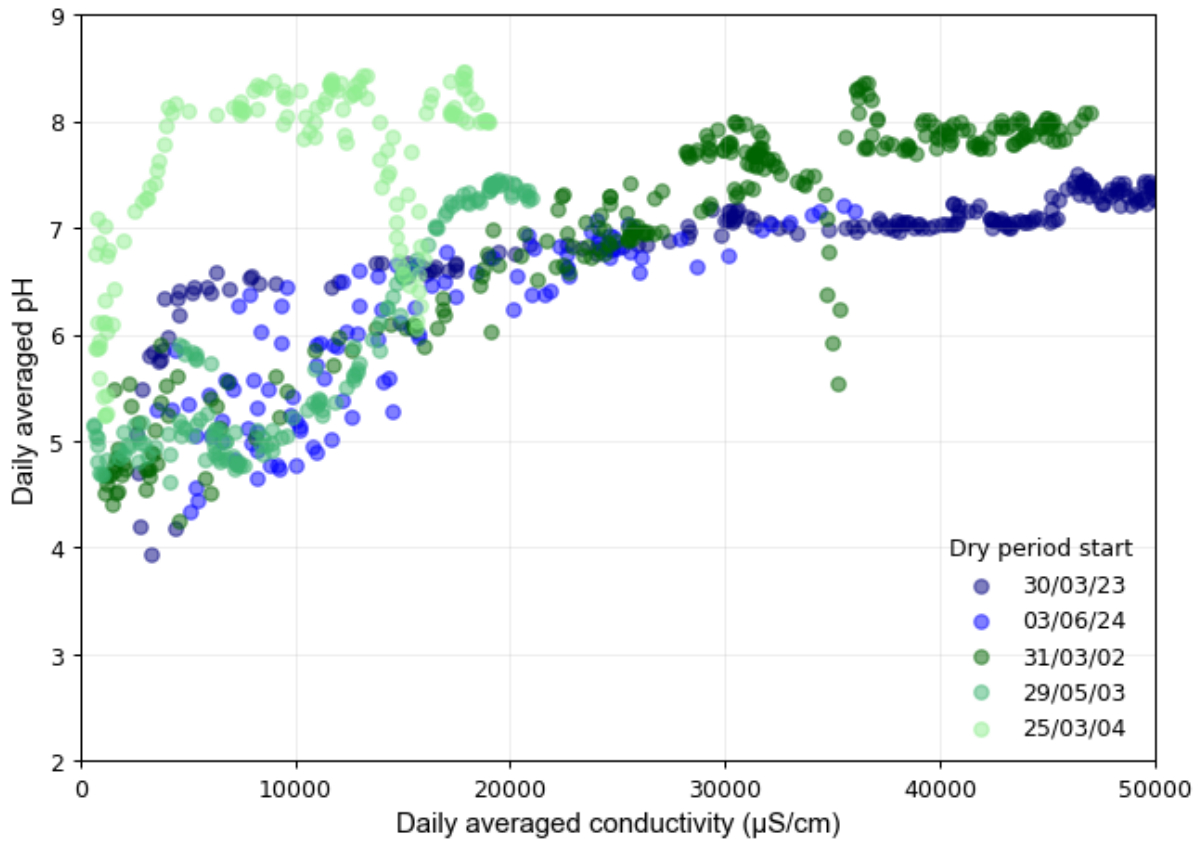
Figure 5-7 Daily averaged pH versus daily averaged conductivity upstream of the Menarcobrinni floodgates for each dry period
