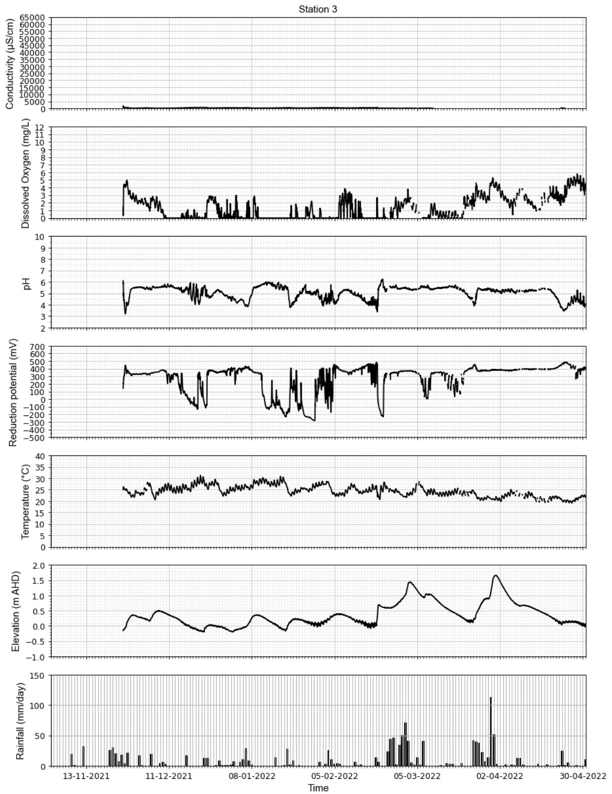
Figure A-14 Water quality data for Station 3 (November 2021 to April 2022)
