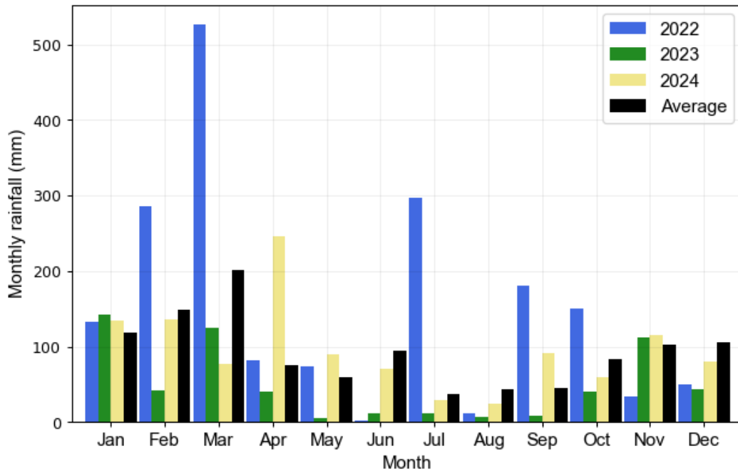
Figure 2-2 Monthly rainfall at Kempsey from 2022 to 2024 (coloured) compared against the average between 2001 and 2025 (black) (data from BOM (2025e))
